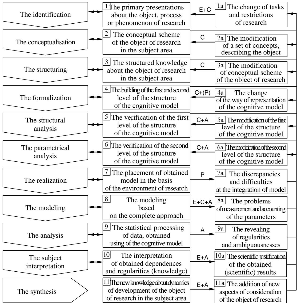
Picture 3.3. The iterative cycle of the cognitive modeling technology
