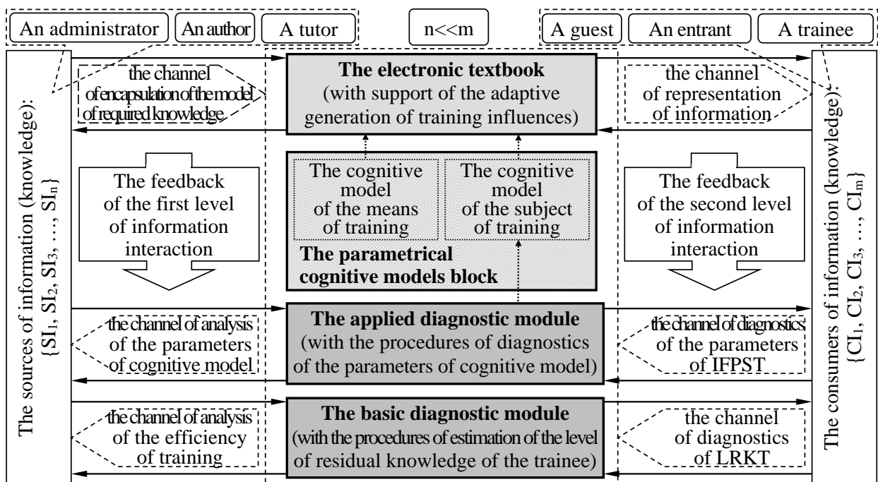
Picture 2.16. The structural scheme of the remote training system with the properties of adaptation
